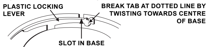
Figure 3b: Removing Sounder From Base
