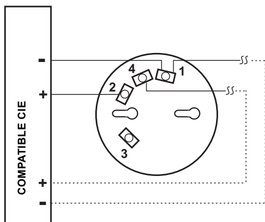
Figure 2: B501AP Wiring
