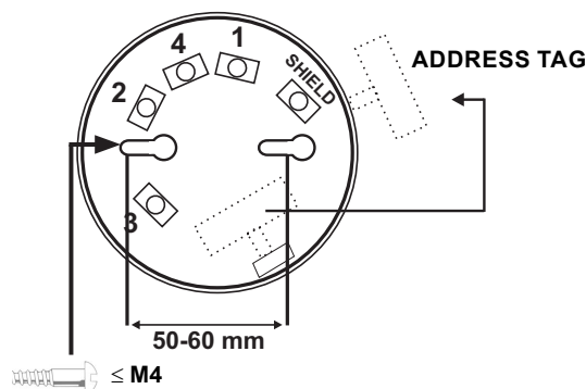
Figure 1: B501AP Mounting
