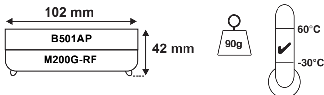
Figure 1: B501AP Mounting
