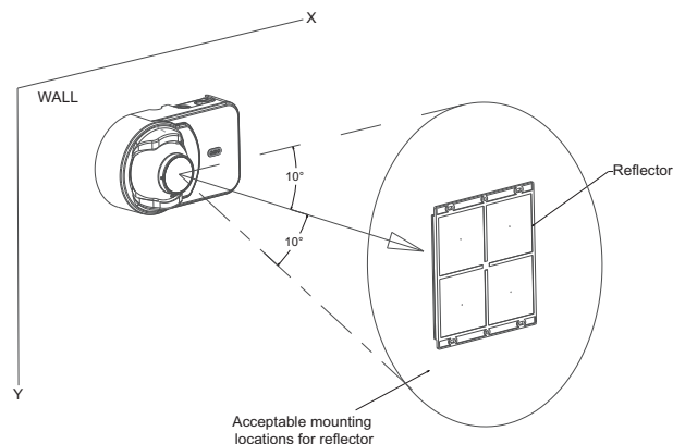
Figure 3-8: Reflector Mounting Guidelines
