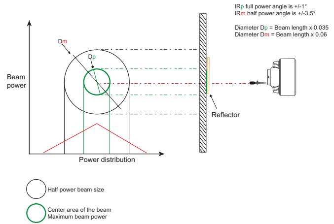
Figure 3-18: Beam Power Distribution
