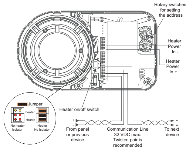
Figure 3-14: Wiring Diagram
