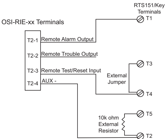
Figure 3-14: Wiring Diagram
