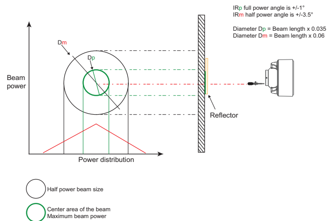
Figure 2-18: Beam Power Distribution
