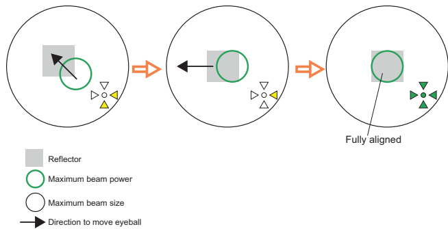
Figure 2-20: Arrow Array Color Alignment Guidance
