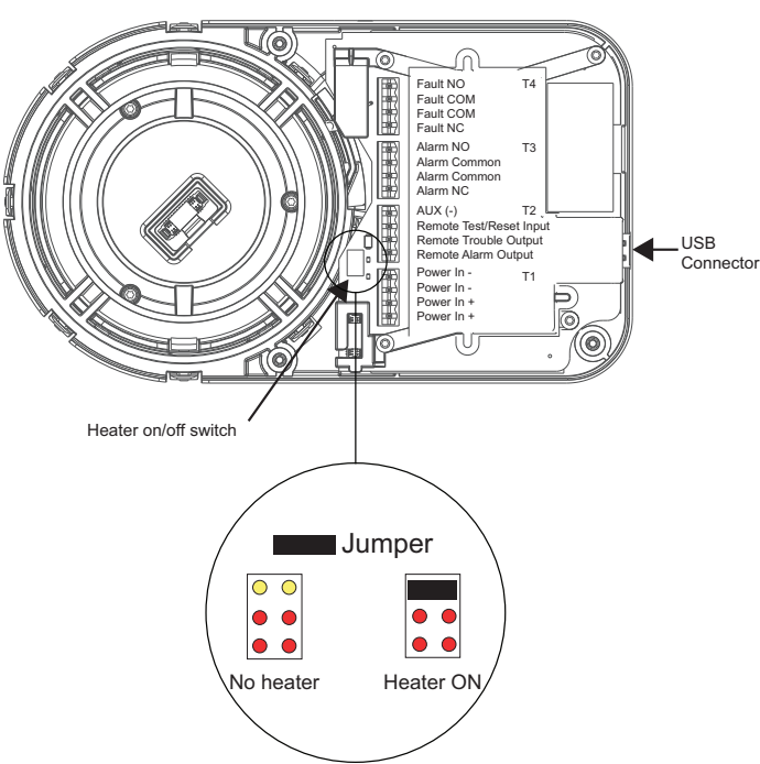
Figure 2-14: Wiring Connections at Detector
