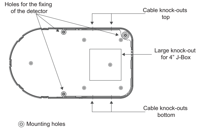
Figure 2-11: Mounting pilot holes
