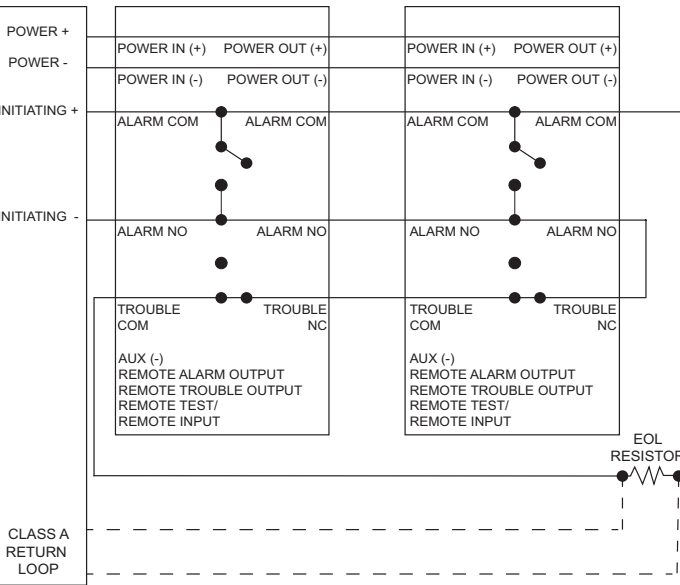
Figure 2-13: Wiring Diagram
