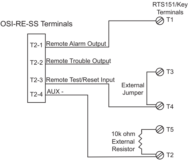
Figure 2-15: Wiring Diagram (RTS451 or RTS151)
