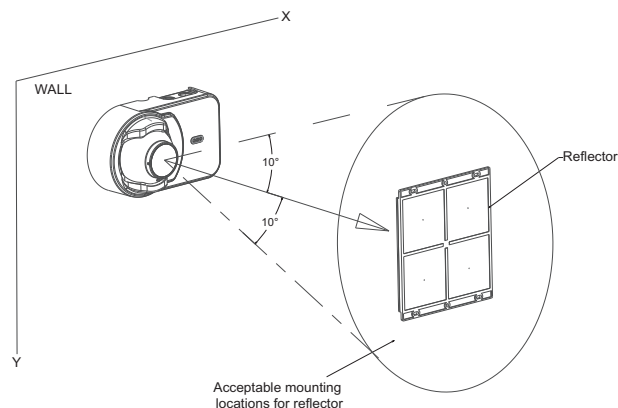
Figure 2-8: Reflector Mounting Guidelines
