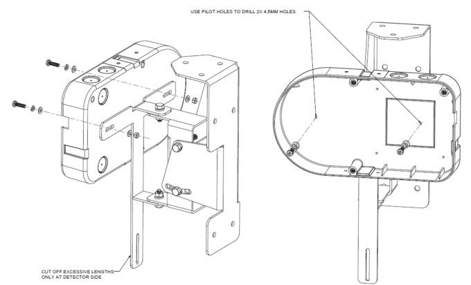
Figure 2-12: Detector Mounting Guidelines
