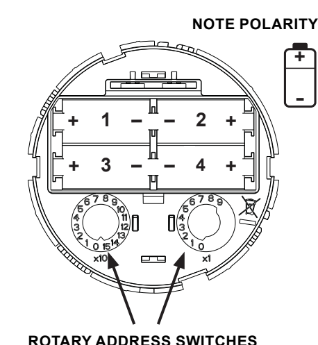
Figure 4: Battery Installation and Rotary Address Switches
