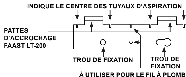
Figure 5: Support de montage
