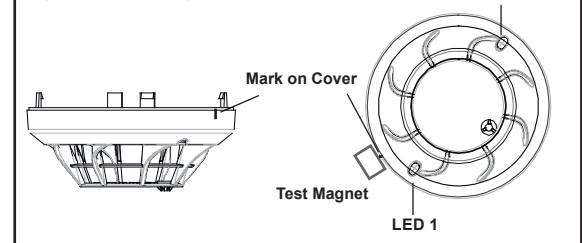
Figure 3: Test Magnet Position
