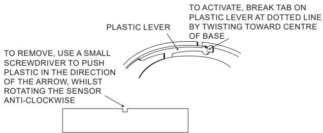
Figure 2: Tamper Resist Feature
