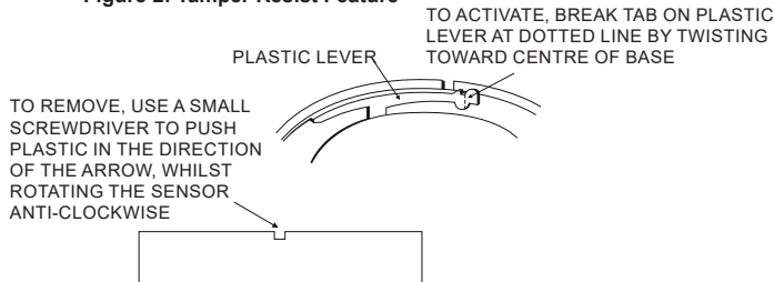
Figure 2: Tamper Resist Feature
