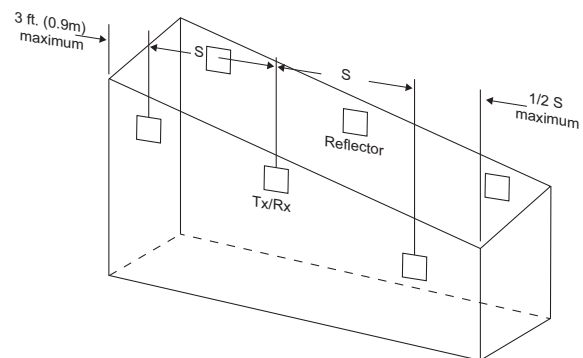
Figure 3-5: Sloped Ceiling (Shed Type)
