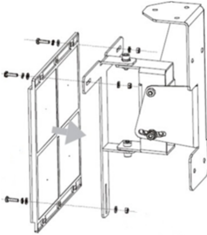
Figure 3-9: Reflector Mounting Guidelines
