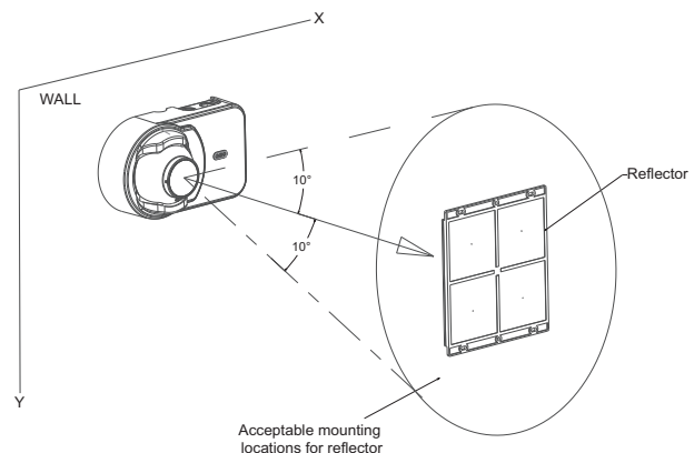
Figure 3-8: Reflector Mounting Guidelines
