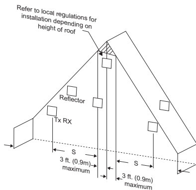
Figure 3-6: Sloped Ceiling (Peaked Type)
