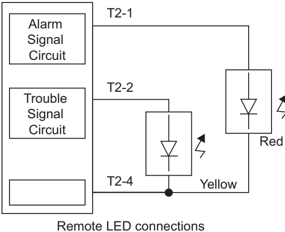
Figure 3-16: Wiring Diagram (Remote LEDs)
