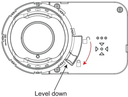
Figure 3-21: Locking and Securing the Eyeball
