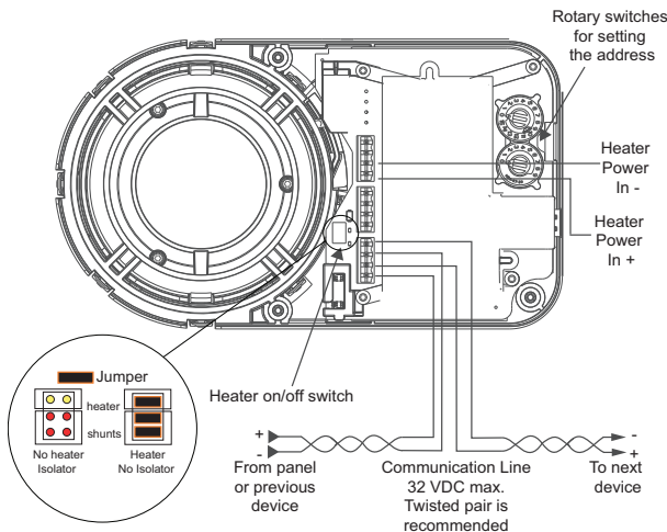
Figure 3-14: Wiring Diagram
