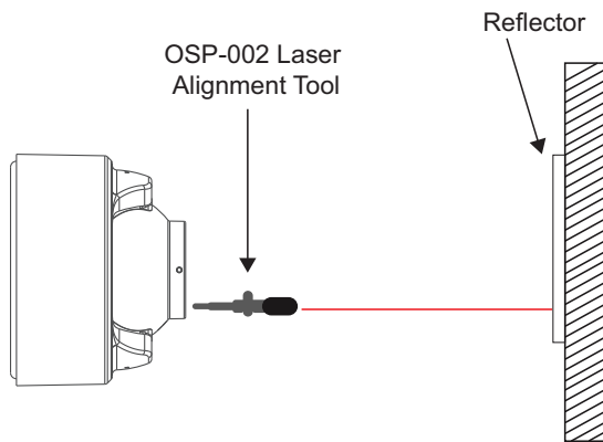
Figure 3-17: Coarse Alignment
