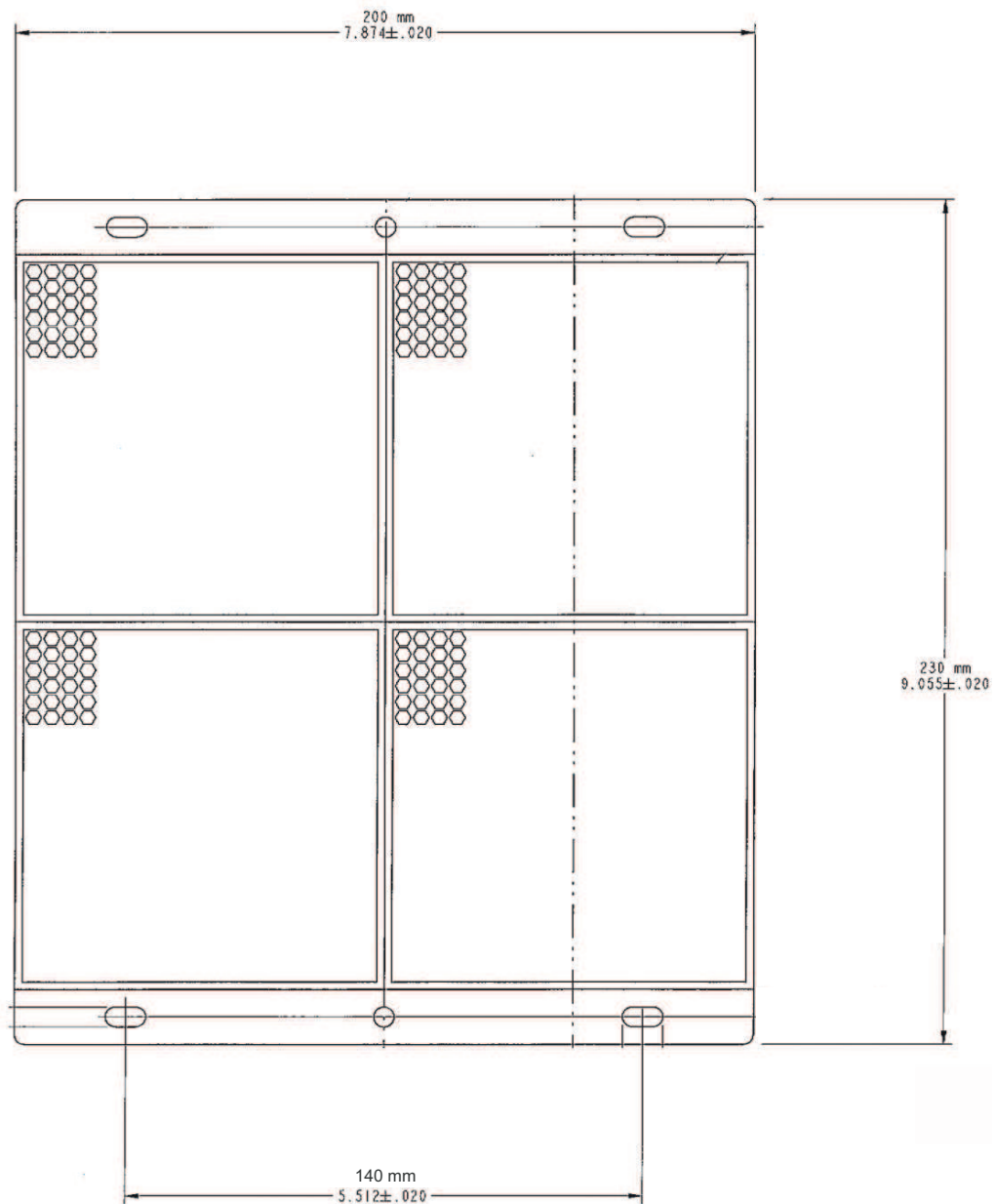
Figure 3-2: Reflector dimensions
