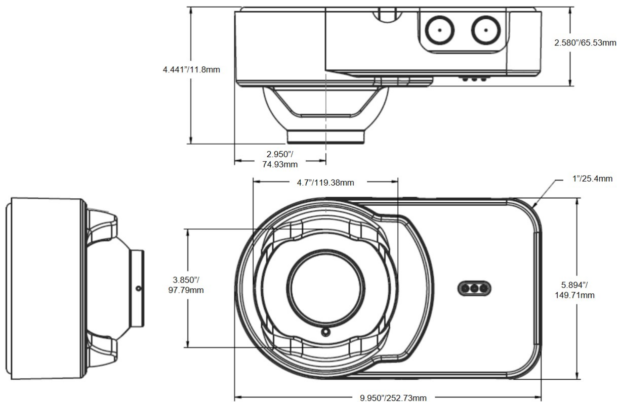
Figure 3-1: Detector dimensions
