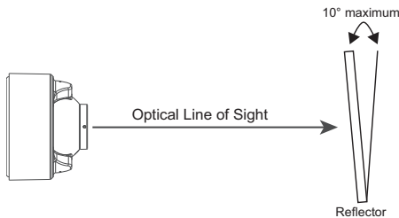
Figure 3-10: Reflector Mounting Guidelines
