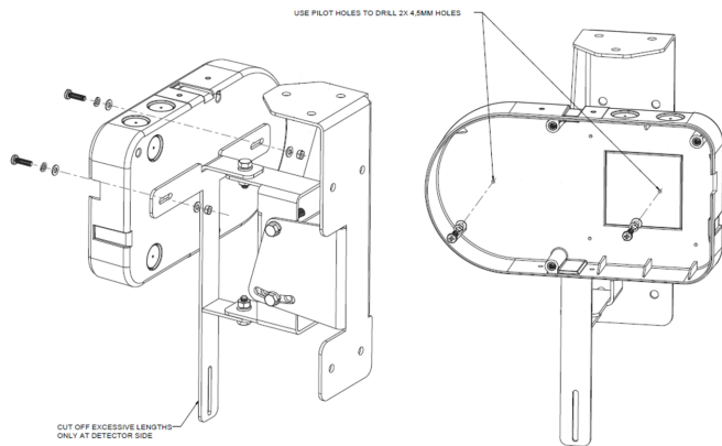
Figure 3-12: Detector Mounting Guidelines
