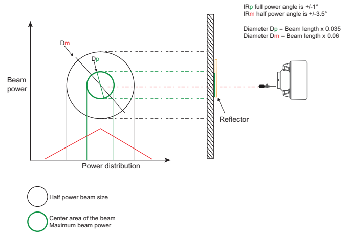
Figure 3-18: Beam Power Distribution
