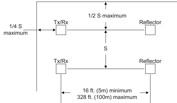
Figure 3-4: Smooth Ceiling (Top View)
