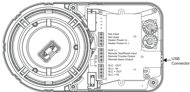
Figure 3-13: Wiring Connections at Detector
