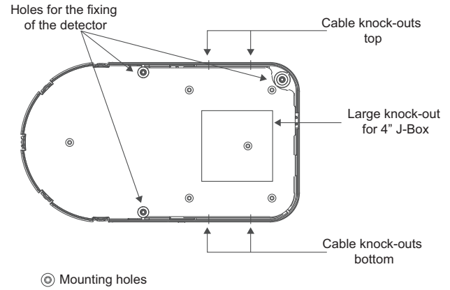
Figure 3-11: Mounting pilot holes
