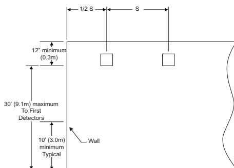
Figure 3-3: Smooth Ceiling (Side View)
