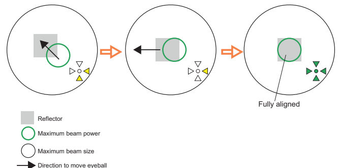
Figure 3-20: Arrow Array Color Alignment Guidance
