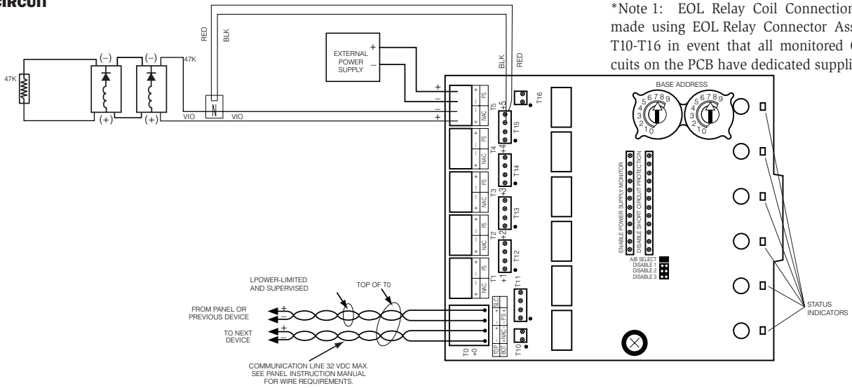
FIGURE 3. CLASS B MONITORED OUTPUT CIRCUIT CONFIGURATION WITH A SINGLE SUPPLY SHARED BY 2 MONITORED OUTPUT CIRCUITS
