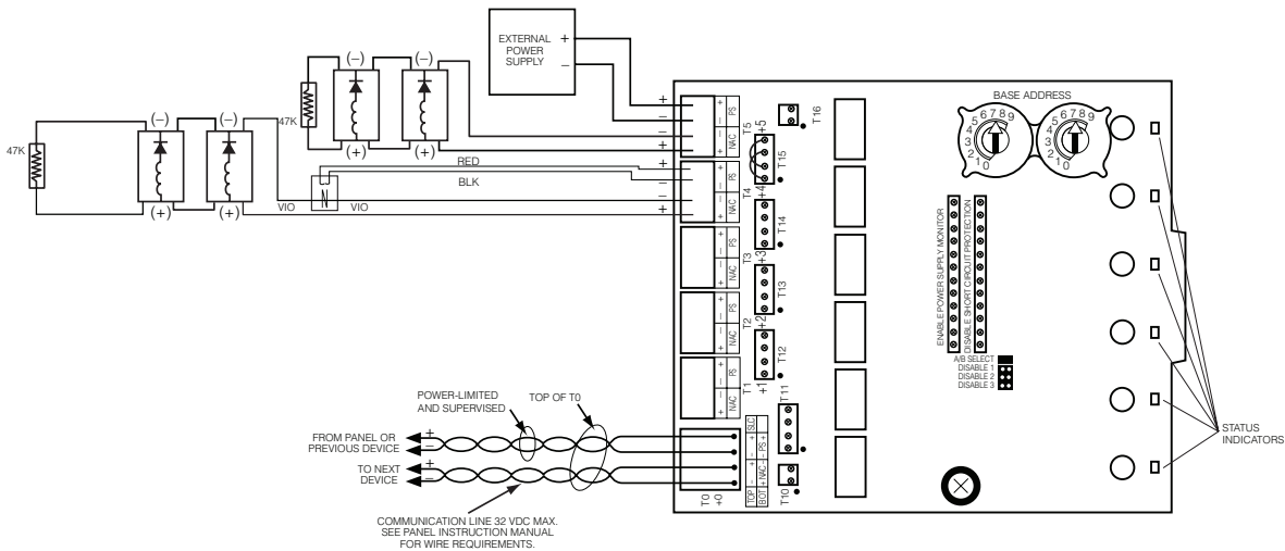
FIGURE 4. EXAMPLE OF MULTIPLE BOARDS SHARING SAME EXTERNAL SUPPLY
