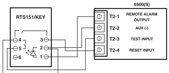
Figure 4: RTS151KEY Wiring
